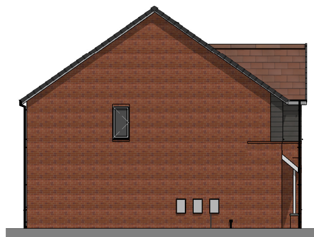
Left Side Elevation. 1 : 150
