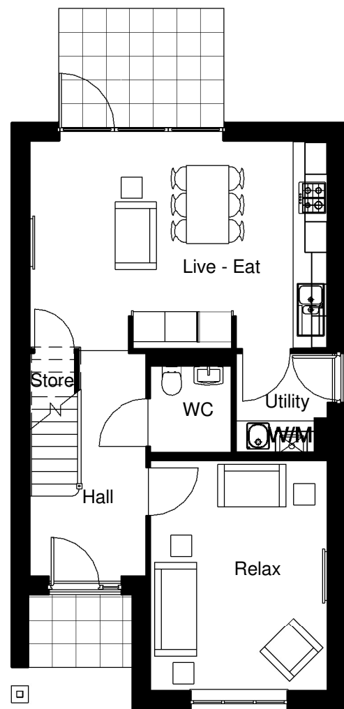
Ground Floor. 1 : 100
